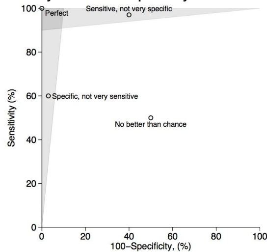
Figure 1. Square plot of sensitivity versus 100%-specificity
