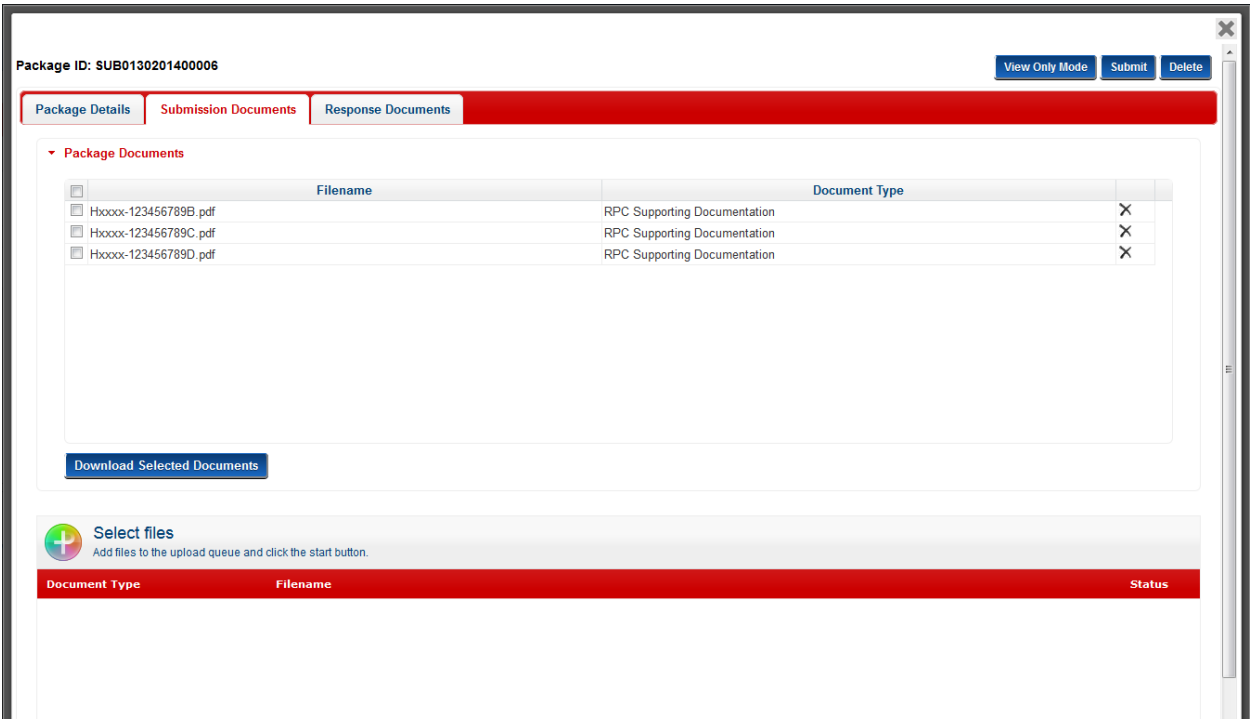
Figure 55: Update Package
