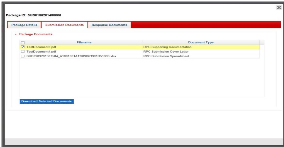
Figure 36: View Package
