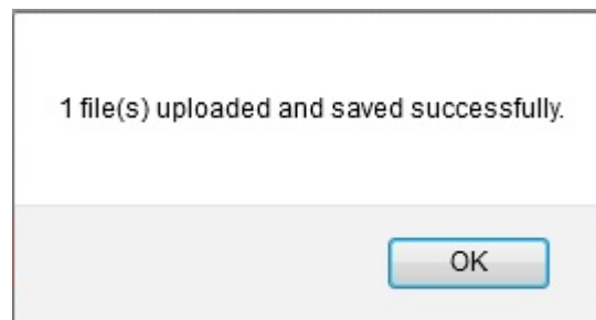
Figure 50: Update Package
