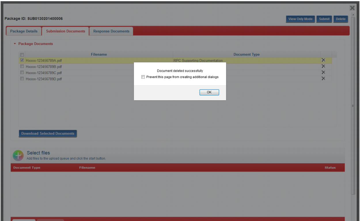
Figure 54: Update Package
