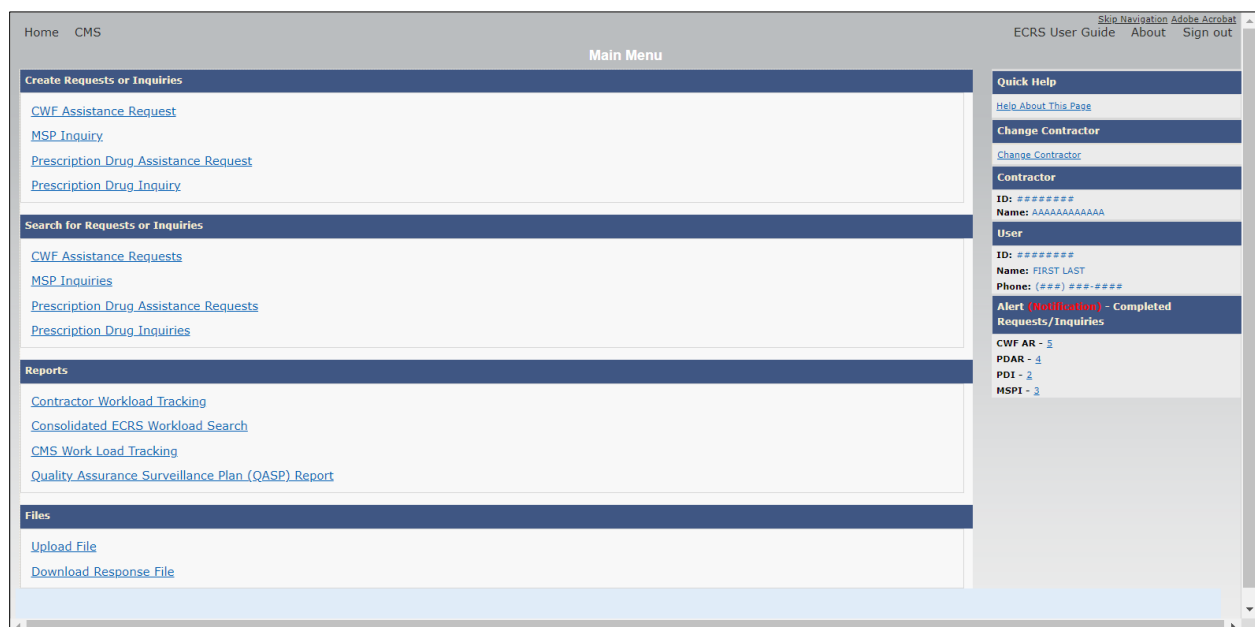
Figure 2-5: Main Menu
