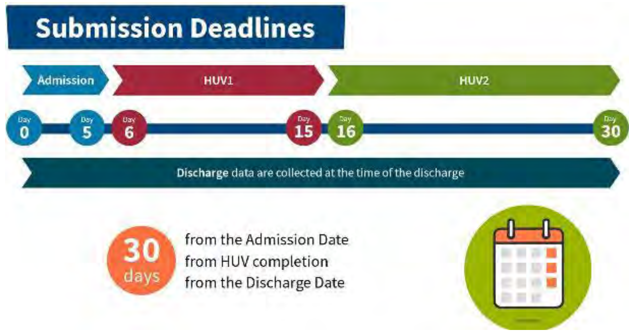
Figure 9: Submission Deadlines
