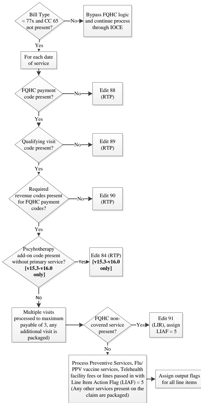
FQHC Processing Logic
