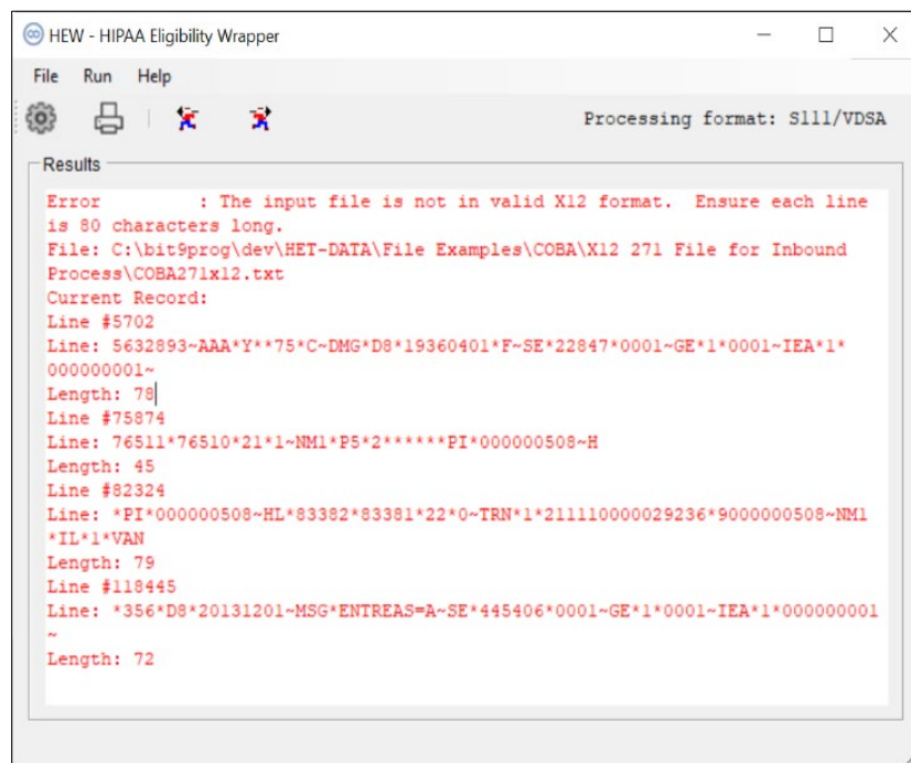
Figure I-14: Completed Inbound 271 S111/VDSA Query (Example)
