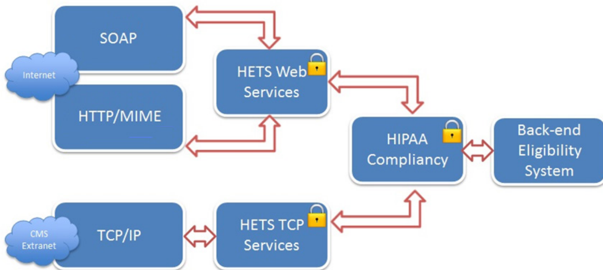
Figure 2 – Transaction Process
