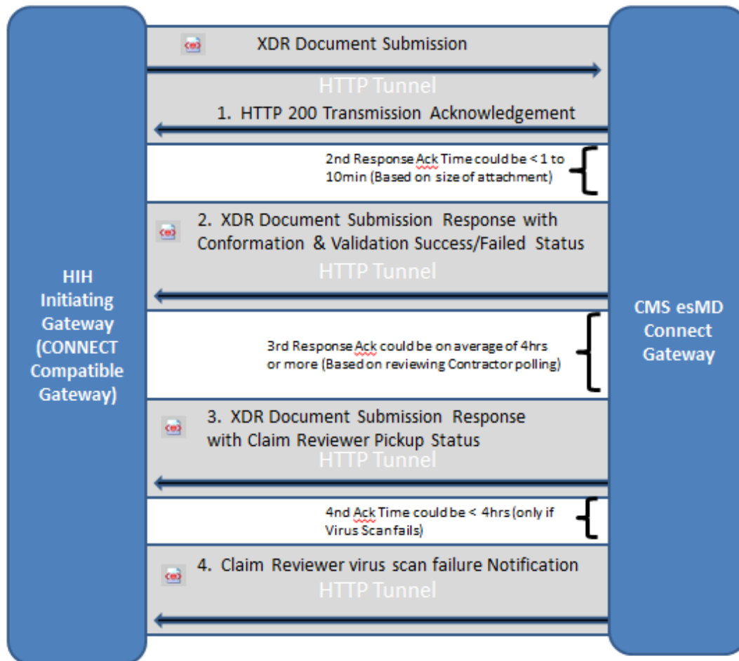
Figure 2: Asynchronous Acknowledgments with Multiple Hyper Text Transfer Protocol (HTTP) Connections
